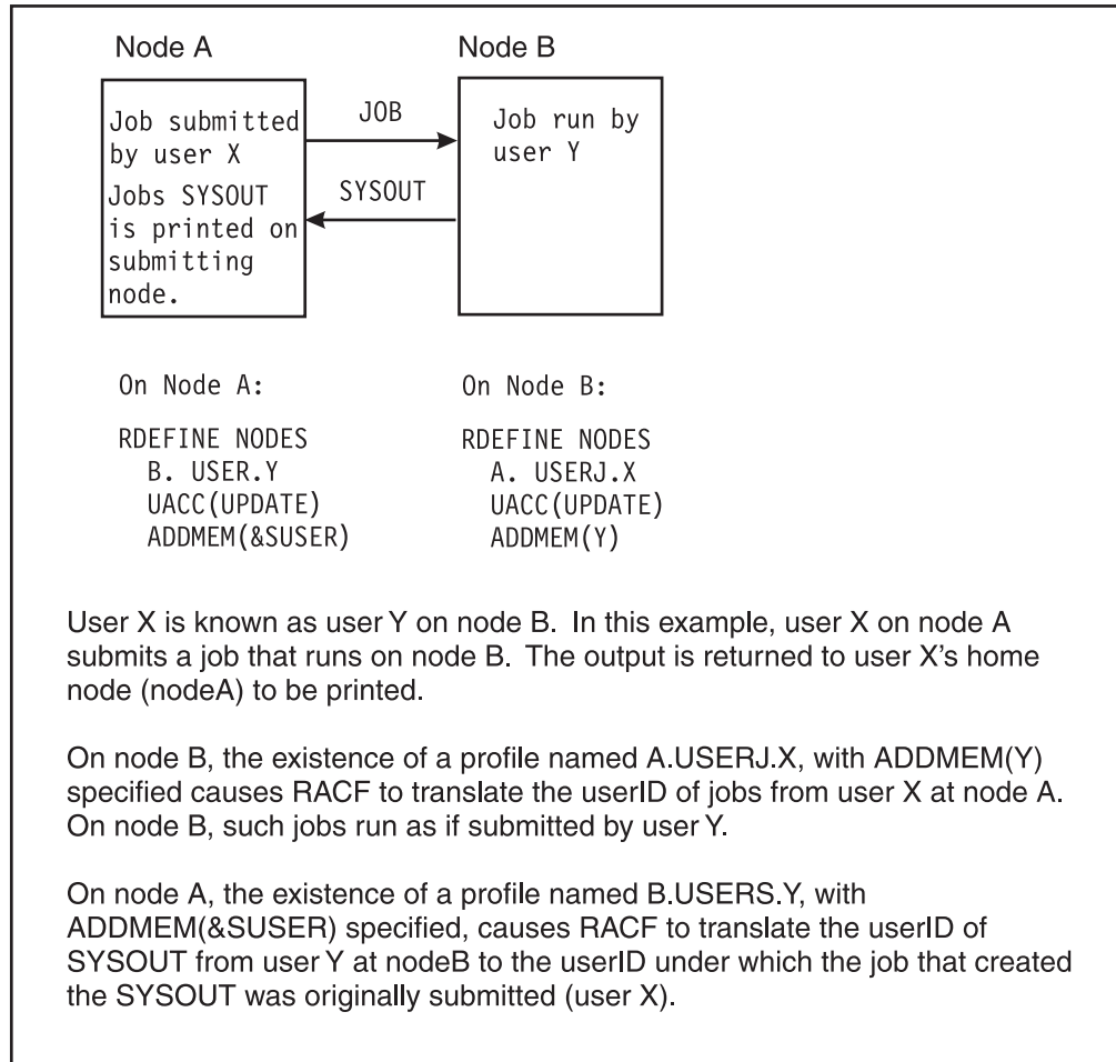
Figure 12. Example: Simple NJE User Translation Using &SUSER
