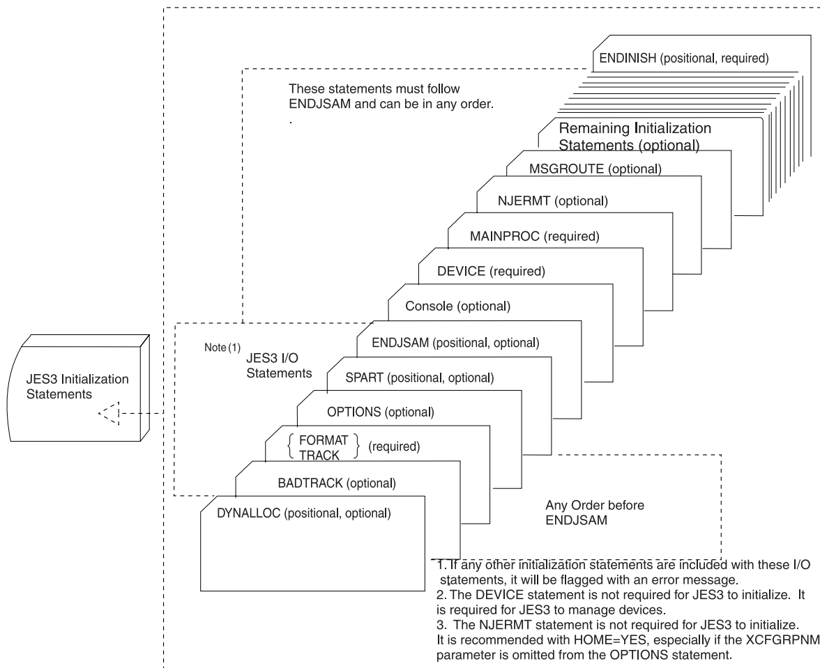
Figure 2. Structure of the JES3 Initialization Stream
