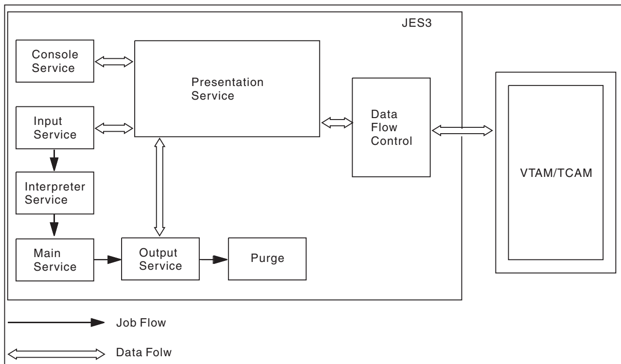
Figure 29. JES3-VTAM Interface
