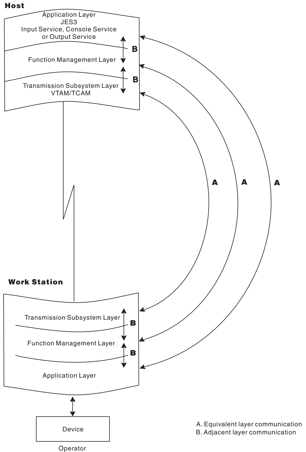
Figure 28. Overview of SNA Environment for JES3
