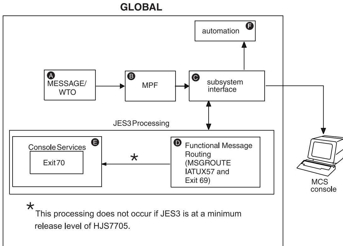
Figure 23. Simplified Path of a Message Issued from a Global Processor
