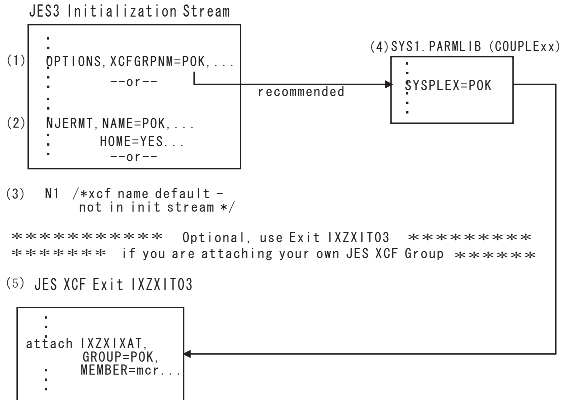
Figure 27. Defining a JES3 XCF Group - Putting the Pieces Together
