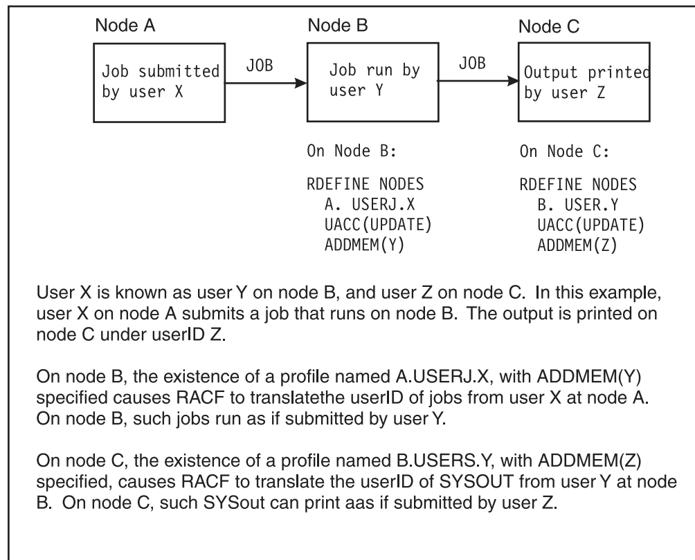
Figure 11. Example: Simple NJE User Translation
