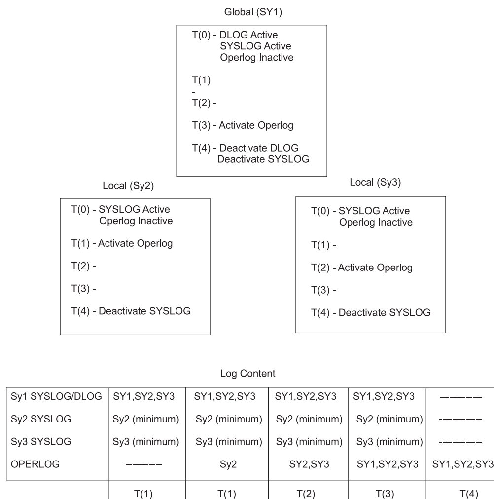
Figure 19. Hardcopy Log Migration Scenario
