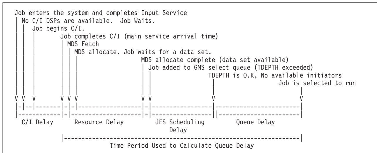
Figure 15. Overview of Pre-Execution Job Delays
