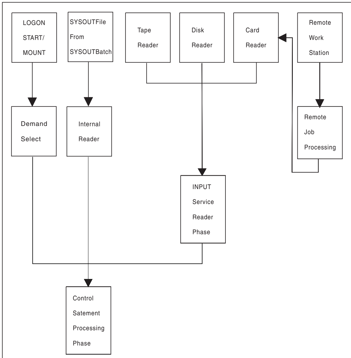
Figure 14. Overview of Job Flow to Input Service
